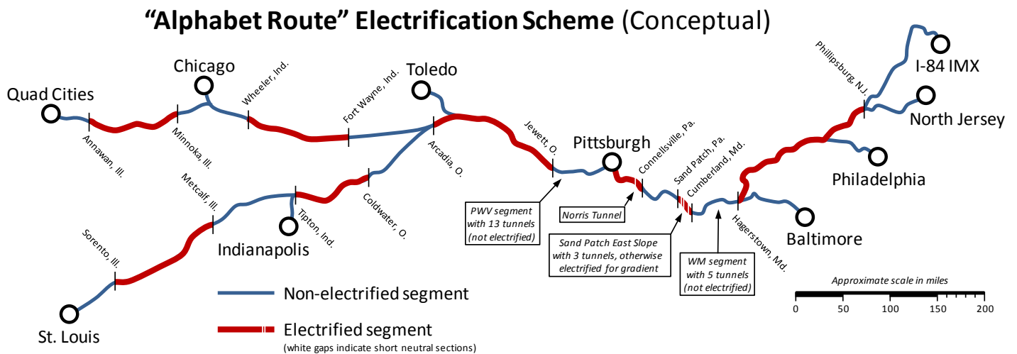
Figure 7. A conceptual illustration of what an intermittent electrification scheme for the consortium known as “Alphabet Route” (with minor additions and subtractions) could look like.
