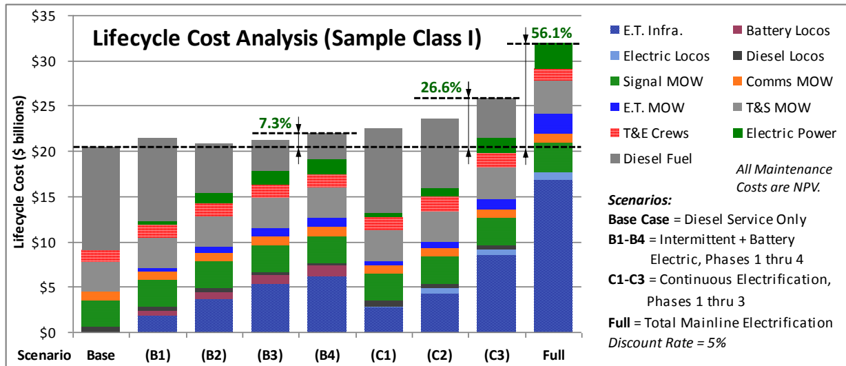
Figure 17. Life Cycle Cost Analysis for a Hypothetical North American Class I Railway
